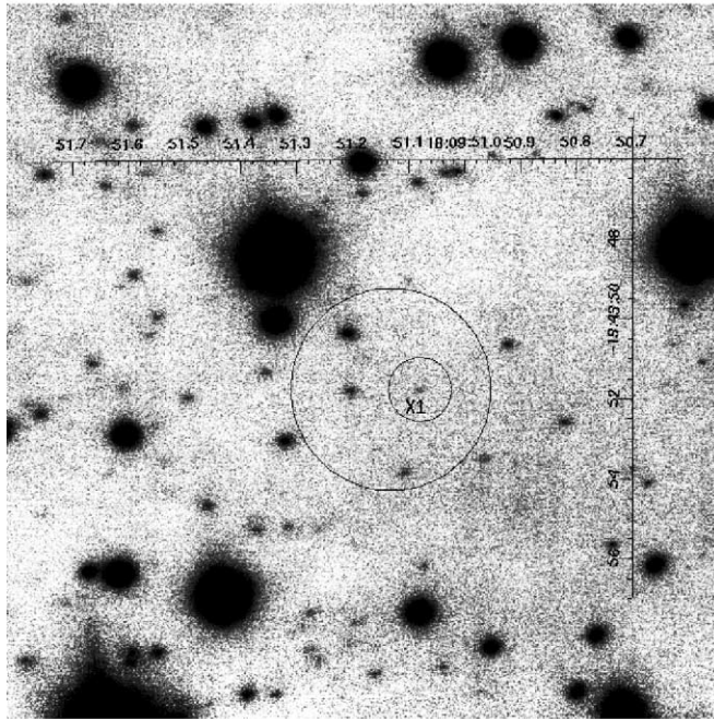
FIG. 1.—Near-IR K' -band image of the region including the position of XTE J1810–197, taken with NAOS-CONICA mounted on VLT UT4 Yepun on 2003 October 7. The two Chandra uncertainty circles ( 2''.5 and 0''.8 radius at 1\sigma and 90% confidence level, respectively) are shown. The proposed IR counterpart is marked with X1. Coordinates are right ascension (hours, minutes, seconds) and declination (degrees, arcminutes, arcseconds; equinox J2000.0).
