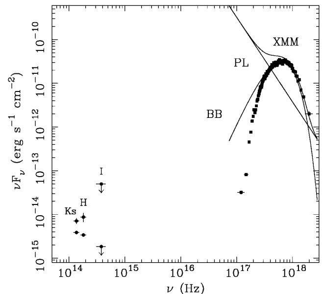
Fig. 2.—Broadband energy spectrum of XTE J1810–197. X-ray raw data are taken from the EPIC-pn instrument on board XMM-Newton (filled squares), while the solid upper curves are the unabsorbed fluxes for the blackbody (BB), the power law (PL), and the sum of the two components. On the lower left corner of the plot are the optical/IR fluxes/upper limits: lower points are absorbed values, while upper points are unabsorbed values for A_V = 5.9 .
